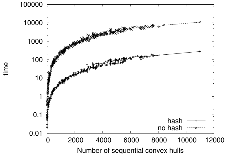
Figure 3: Run-time (in seconds) performance of hashing determinants method for a number of sequential convex hull operations.
