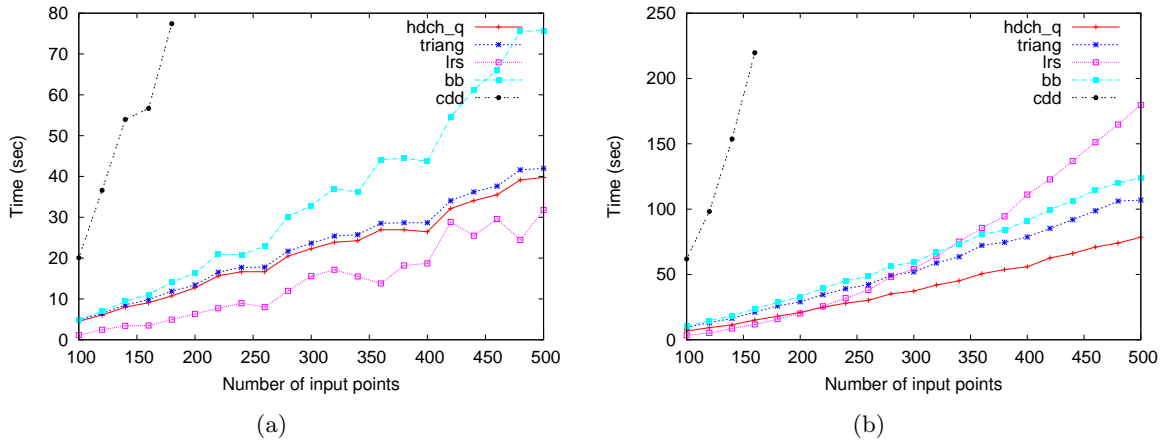
Figure 2: Comparison of convex hull packages for 6-dimensional inputs with rational coefficients. Points are uniformly distributed (a) inside a 6-ball and (b) on its surface.
