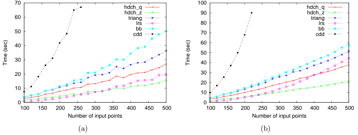
Figure 1: Comparison of convex hull packages for 6-dimensional inputs with integer coefficients. Points are uniformly distributed (a) inside a 6-ball and (b) on its surface.
